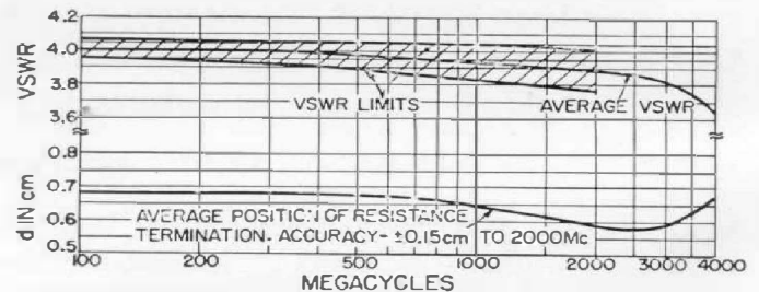
sistance termination as indicated in Figure 1. The cross-lined area indicates the tolerances on the characteristics.
