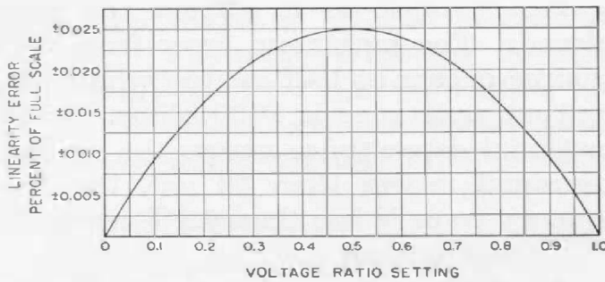
Figure 4. Maximum error in per cent of full-scale maximum setting.
