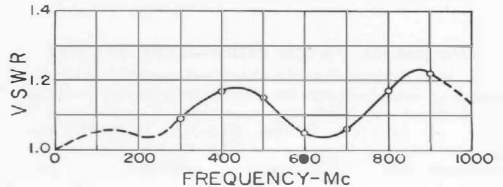
Figure 4. Plot of the VSWR at the 300-ohm terminals of a typical Type 874-UB-P3 Terminal Pad as a function of frequency when the pad is inserted in a properly adjusted balun whose coaxial circuit is terminated in 50 ohms.
