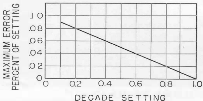
Figure 3. Maximum error as a function of scale setting.
