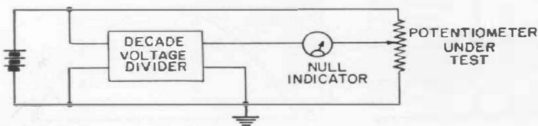
Figure 7. Voltage divider in null circuit for linearity tests.
