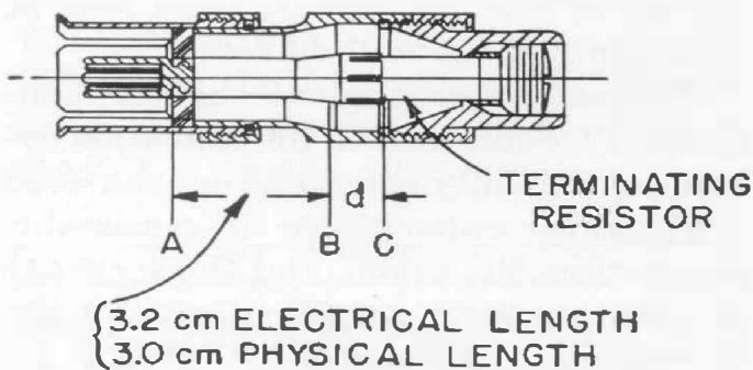
Figure 1. Cross sectional view of Types 874-W100 and W200 Coaxial Standards. The effective position of the pure resistance termination is at C. Type 874-WN and WO Short and Open-Circuit Termination Units effectively terminate a line at A and Type 874-WN3 and WO3 3cm Short and Open-Circuit Termination Units effectively termi-
