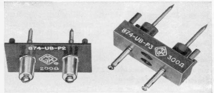
Figure 3. Type 874-UB-P2 Balun Terminal Unit (200 ohms) and the Type 874-UB-P3 300-Ohm Balun Terminal Pad.
