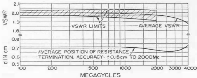
Figure 2a. Plot of the VSWR and position of the pure resistance termination, for a Type 874-W100 100-Ohm Coaxial Standard. The distance, d, is the distance from the position of the short or open circuit produced by a Type WN3 or WO3 Termination Unit to the position of the pure re-
