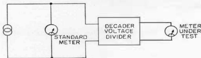
Figure 8. Circuit for calibration and test of vacuum-tube voltmeters.
