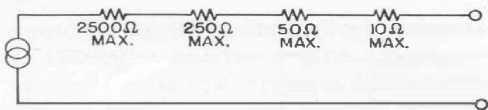
Figure 6. Equivalent circuit of a four-decade divider.
