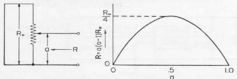
Figure 5. Output resistance characteristic of a simple voltage divider.
