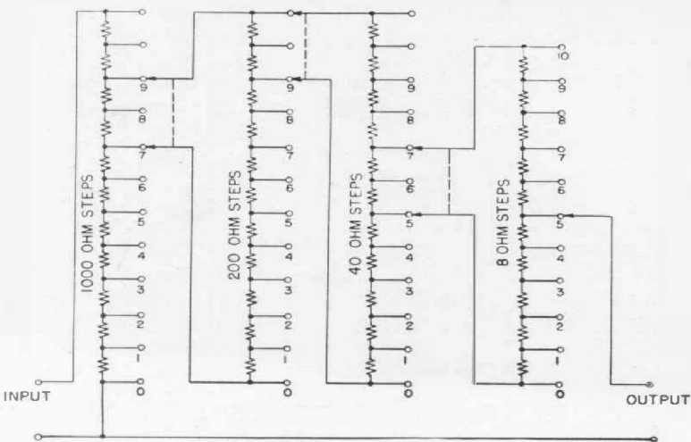
Figure 2. Schematic diagram showing the method of voltage division.
